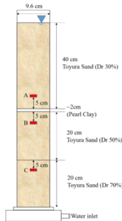
Figure 7: Schematic diagram of experimental setup.
